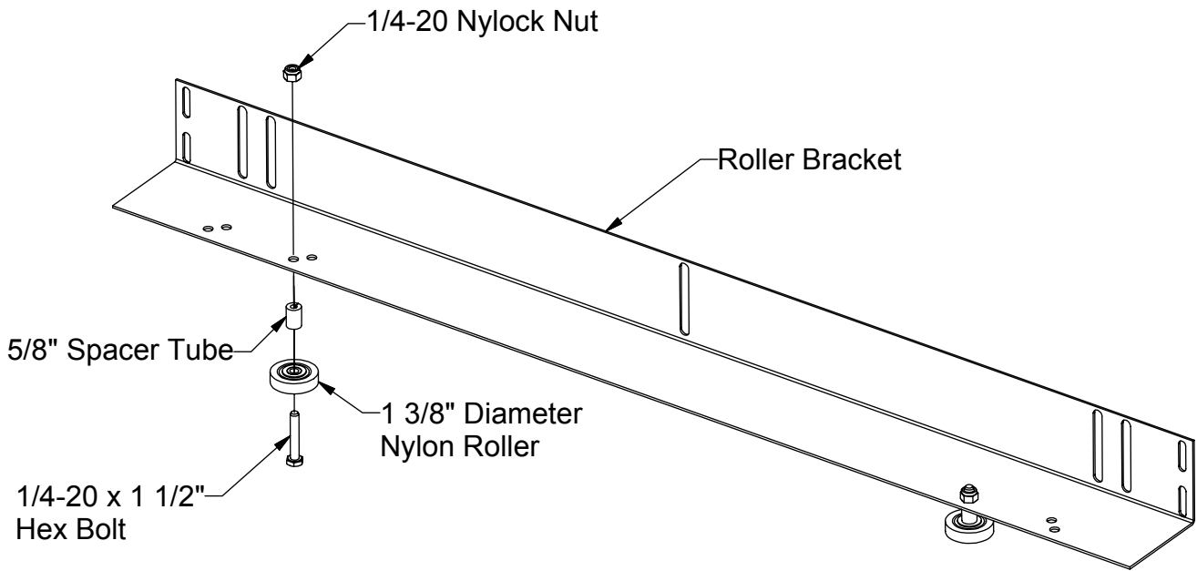
Standard BiSlider with 4" overtravel
