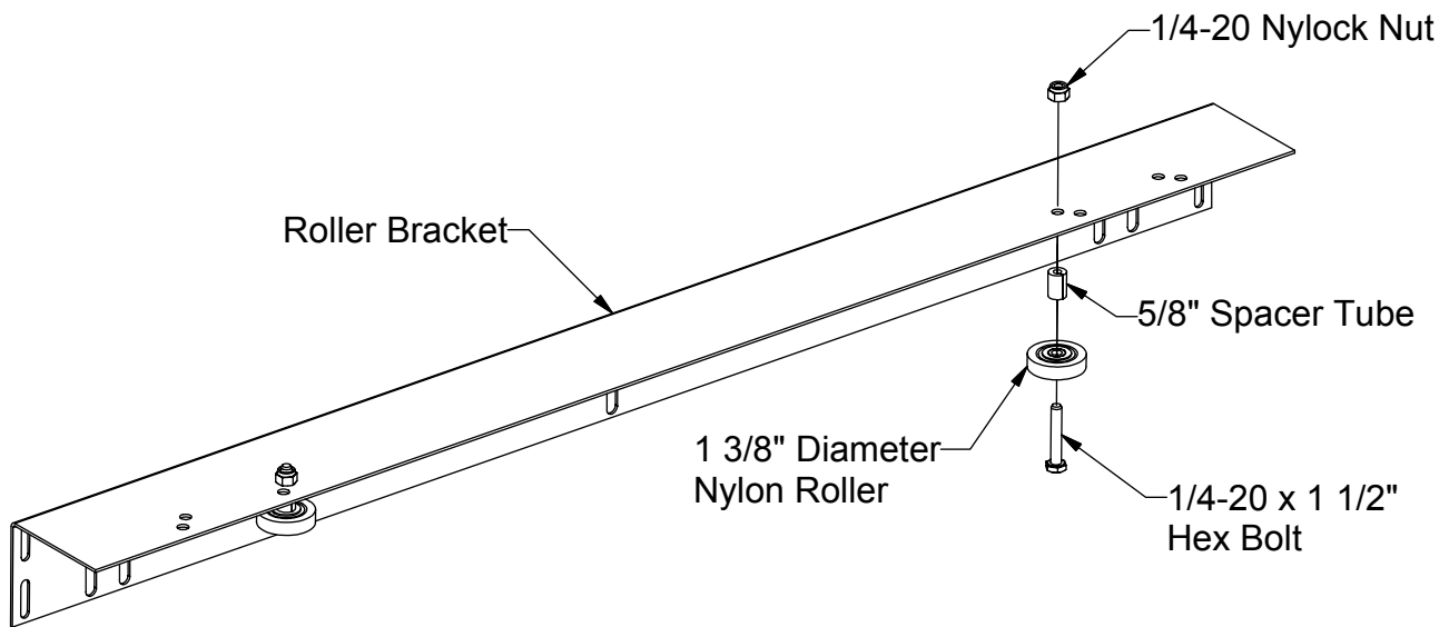
4Post BiSlider with 4" overtravel
