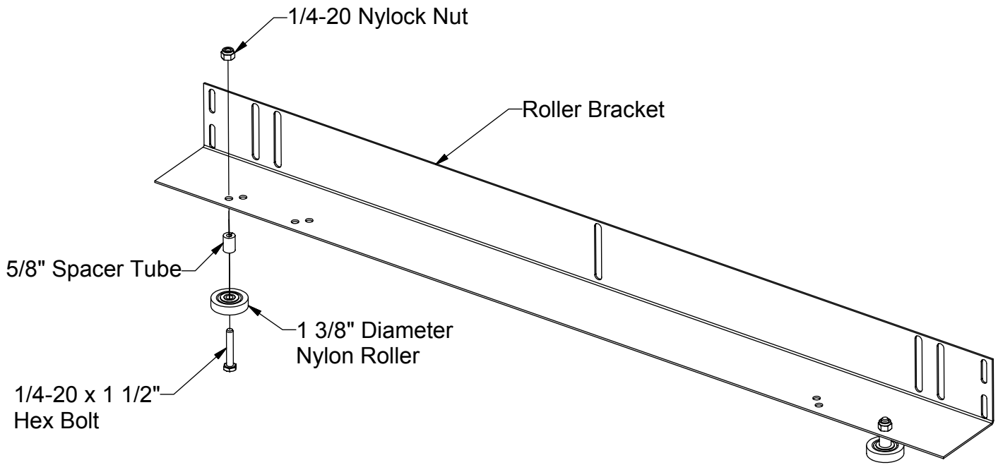
Standard BiSlider with 0"- 2" overtravel
