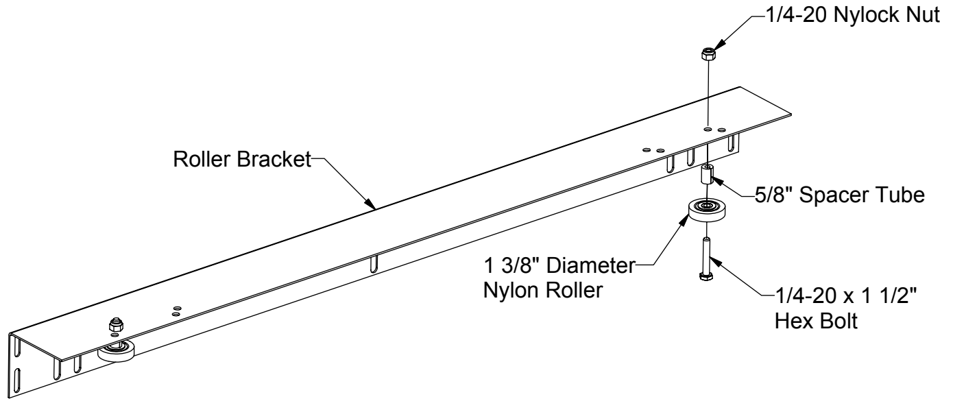
4Post BiSlider with 0" - 2" overtravel
